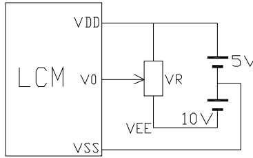
(b) Without DC/DC
