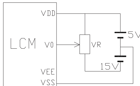
(b) Double Power Without DC/DC
