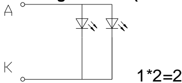
LED Backlight circuit (color: White)
