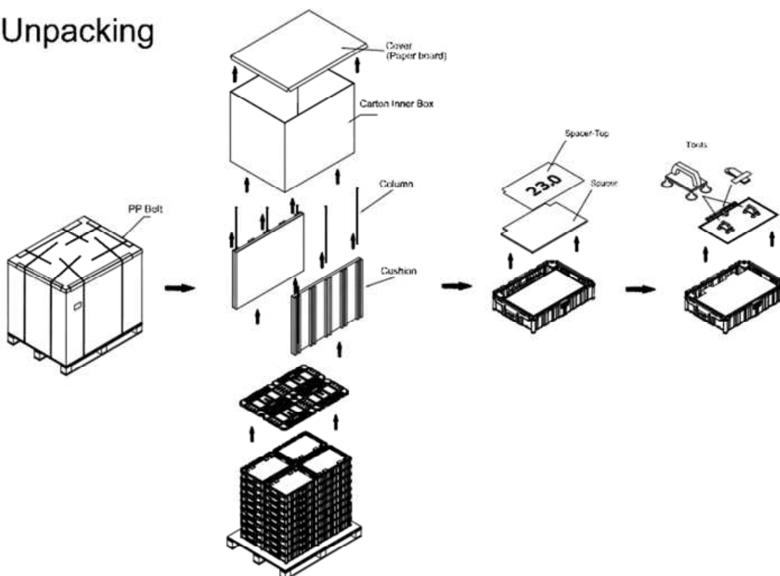
Figure. 8-3 unpacking method
