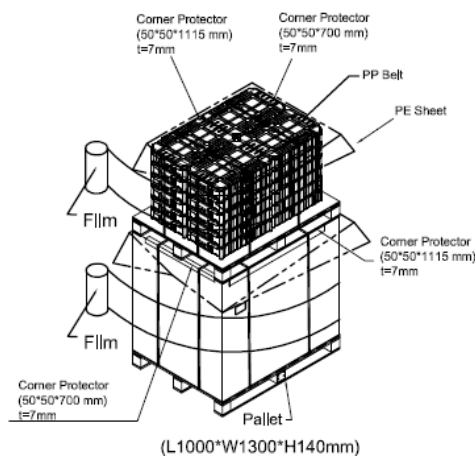
Figure. 8-2 packing method
