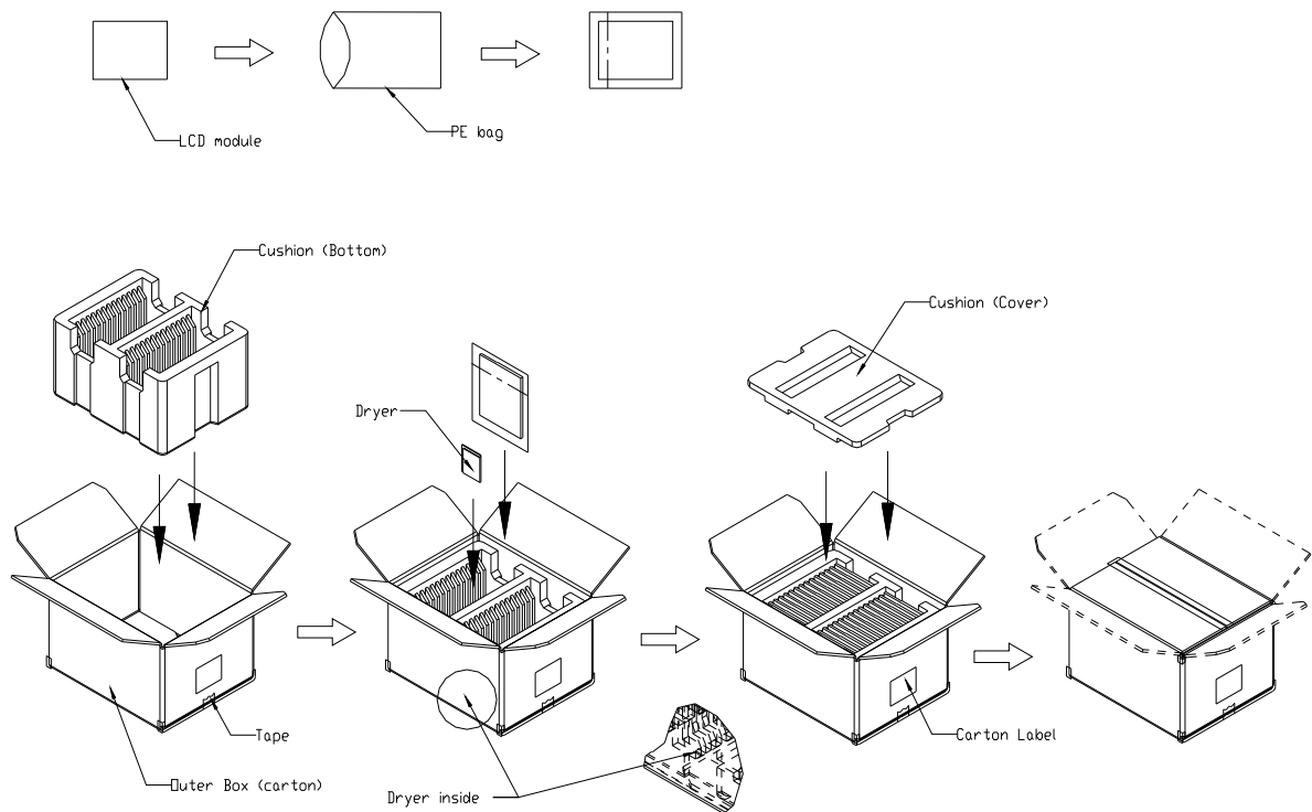
Figure.9-1 packing method
