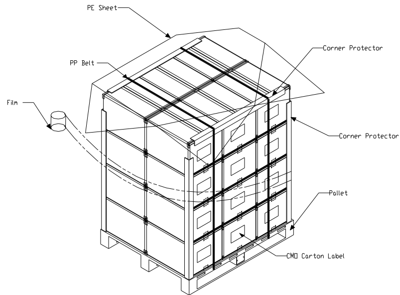
Figure. 9-2 Packing method
