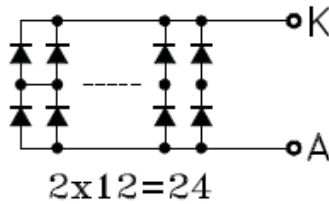
BACKLIGHT CIRCUIT DIAGRAM(COLOR :Yellow-Green)
