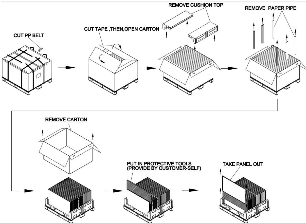
Figure 10-3 un-packaging method
