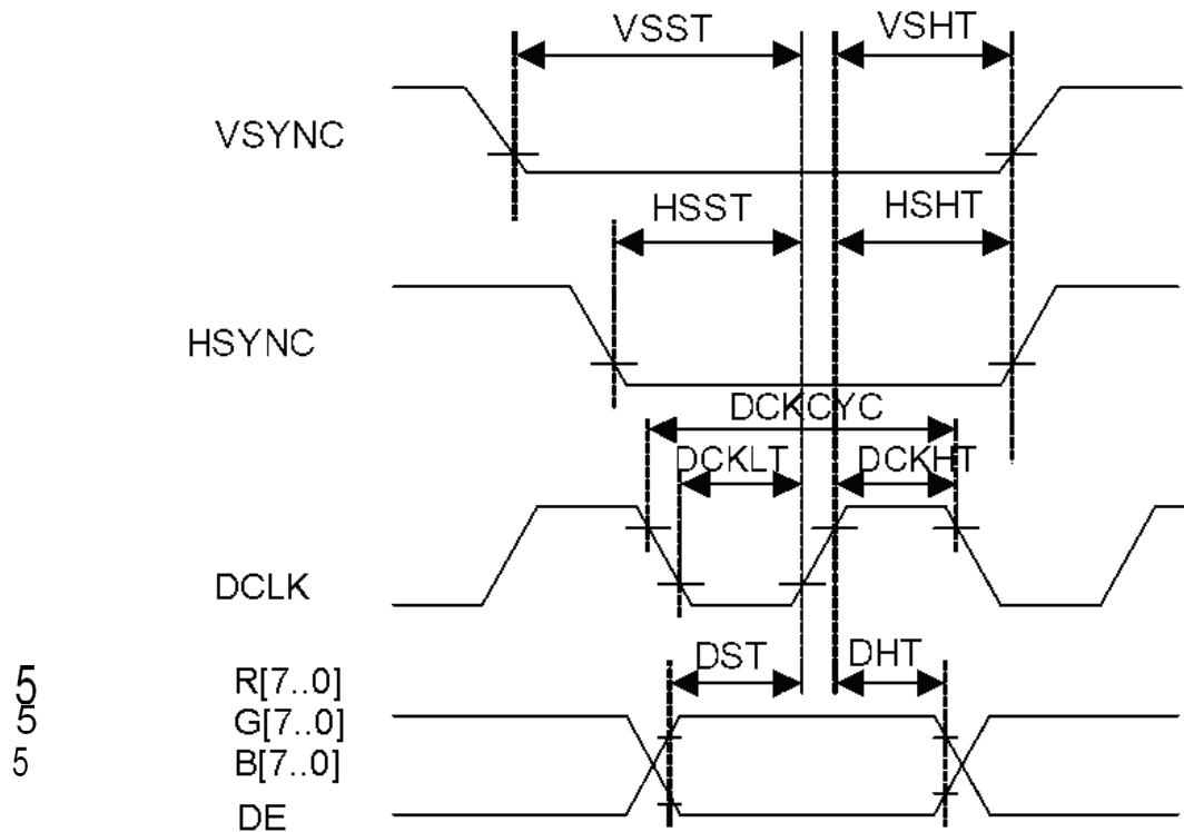
Figure 5.2.3.1 General Timings for RGB I/F
