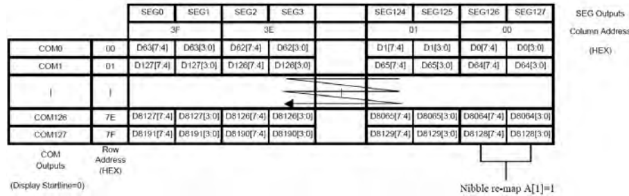
GDDRAM address map 3
