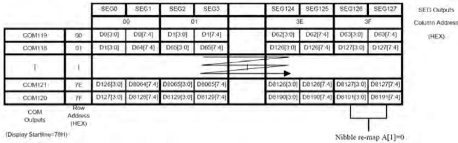
GDDRAM address map 4
