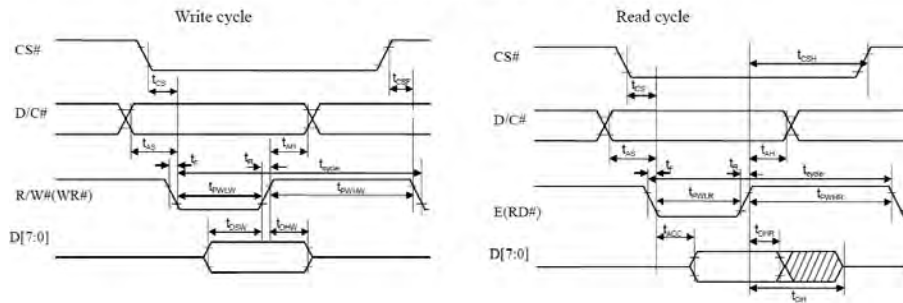
8080-series MCU parallel interface characteristics
