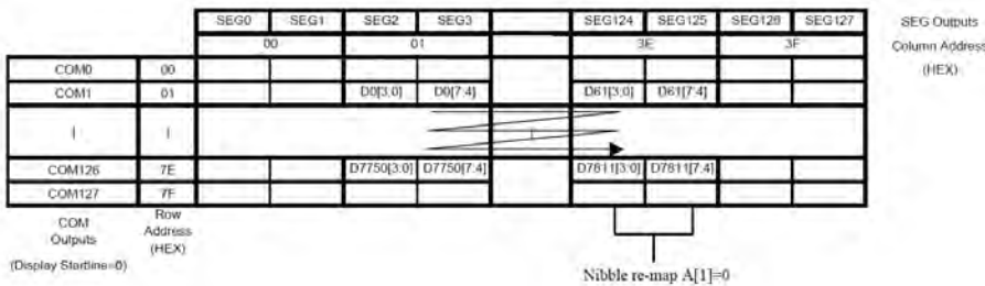
GDDRAM address map 5
