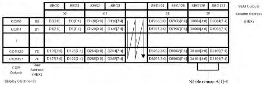
GDDRAM address map 2
