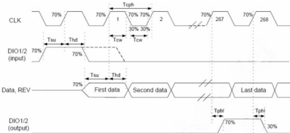
■ Timing Diagram 1
